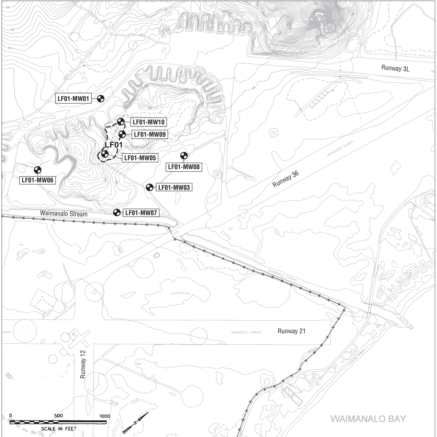
Figure 11 Long-Term Monitoring Well Network for Alternative 3 EE/CA FOR SITE LF01, BELLOWS AFS
