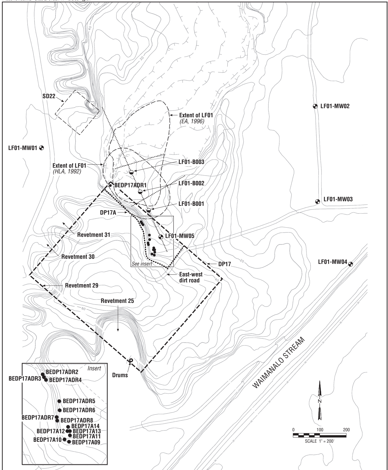
Figure 1-3 Sites LF01 and DP17: Previous Investigations Bellows AFS OU1 EE/CA
