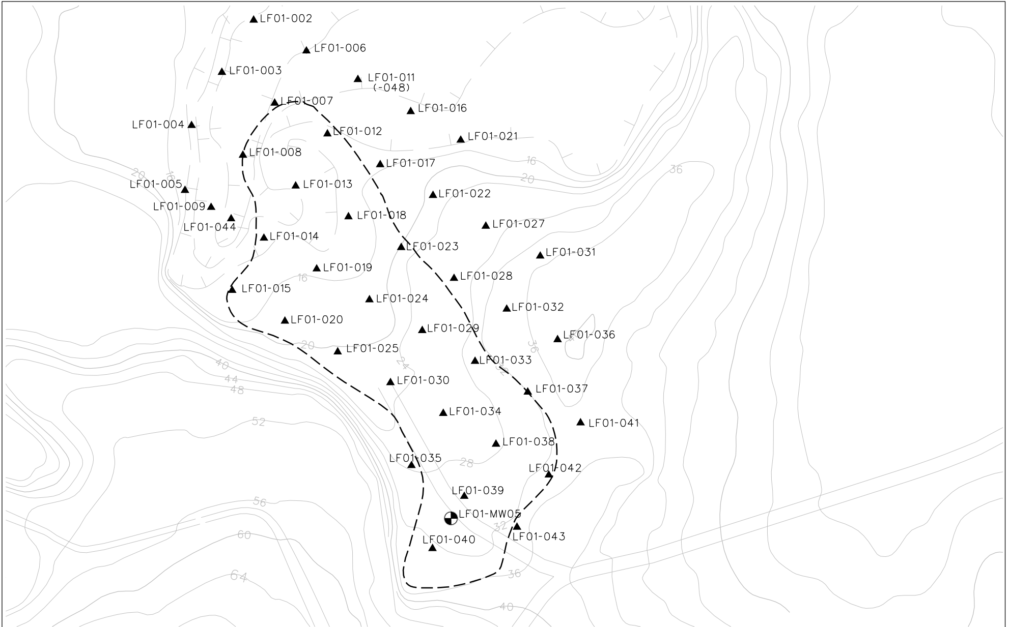
Figure 2-1 Site LF01: Passive Soil Gas Sampling Locations Bellows AFS OU1 EE/CA
