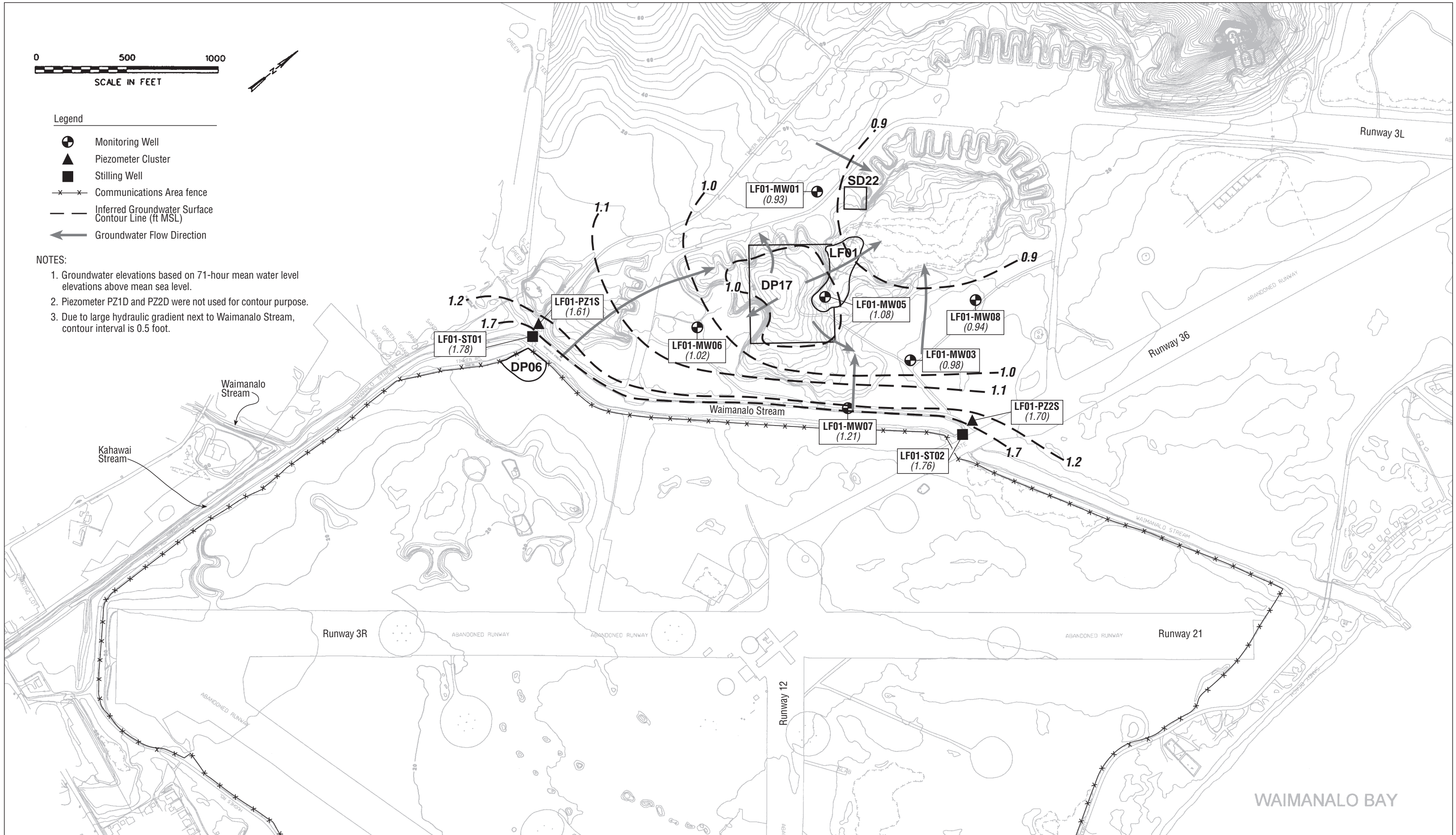
Figure 3-3 Site LFO1: Upper Aquifer Groundwater Contour Map Bellows AFS OU1 EE/CA
