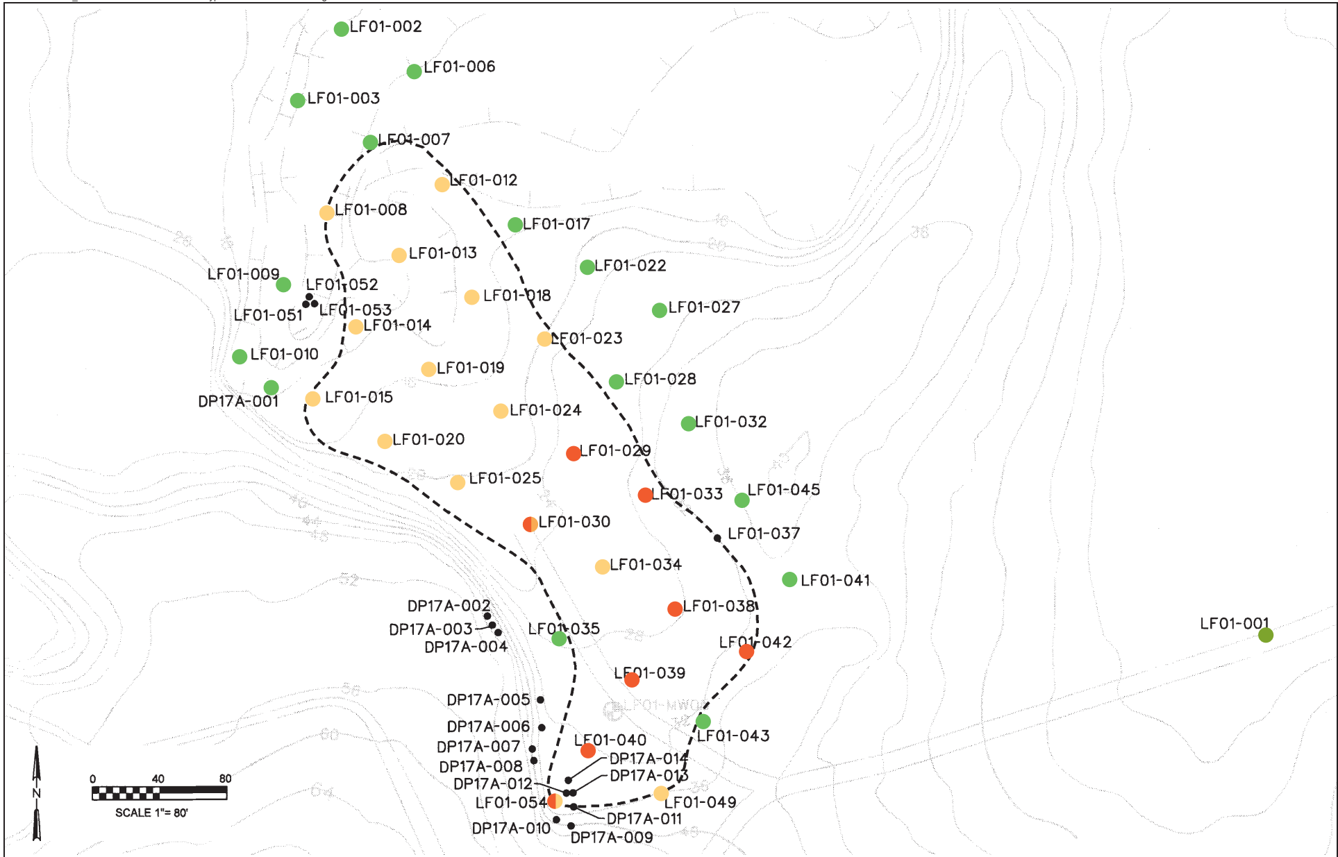
Figure 4-1 Site LF01: Generalized Waste Types and Horizontal Extent of Landfilled Materials Bellows AFS OU1 EE/CA
