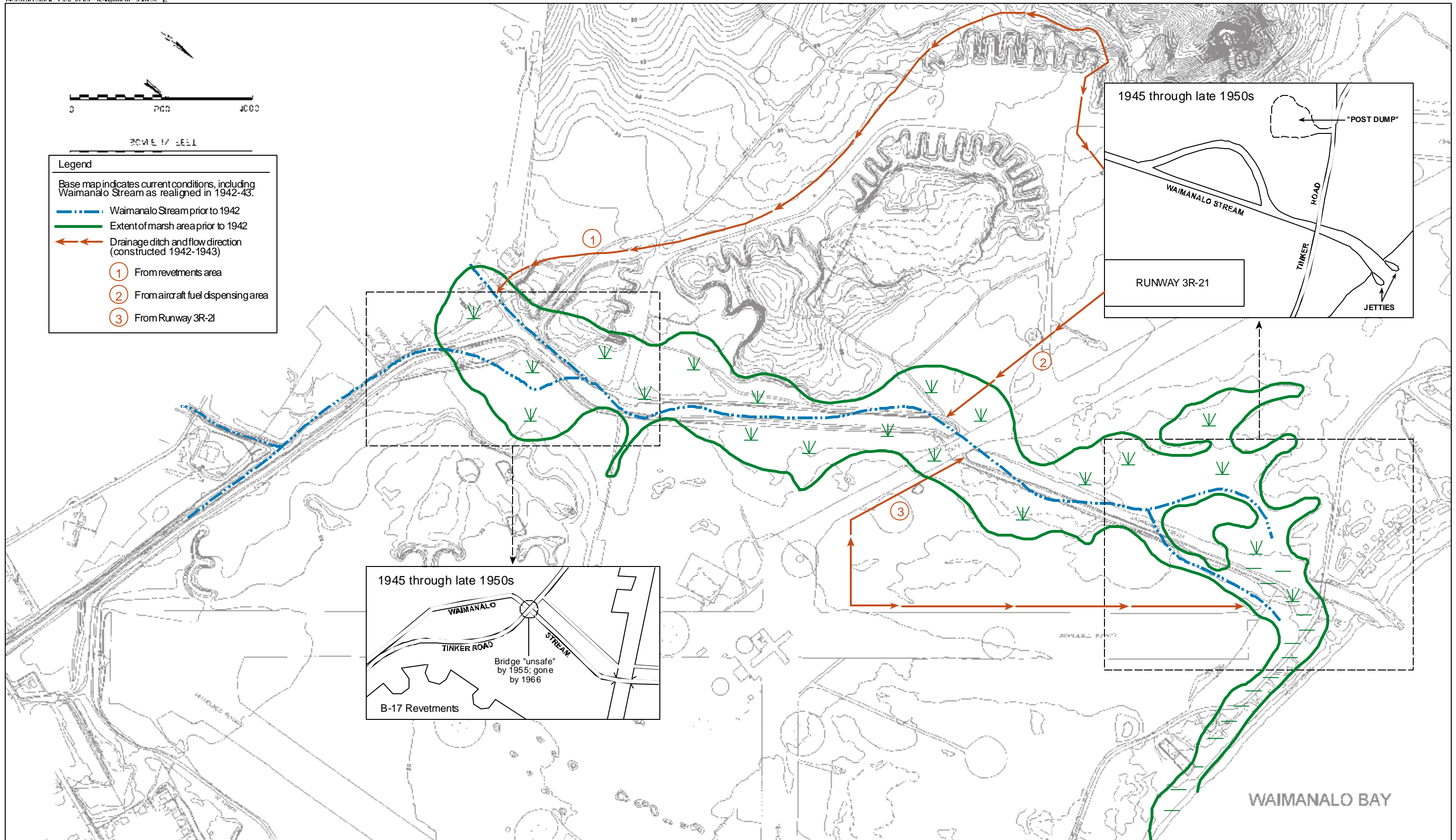
Figure 5-5 Waimanalo Stream Realignment Bellows AFS OU1 EE/CA
