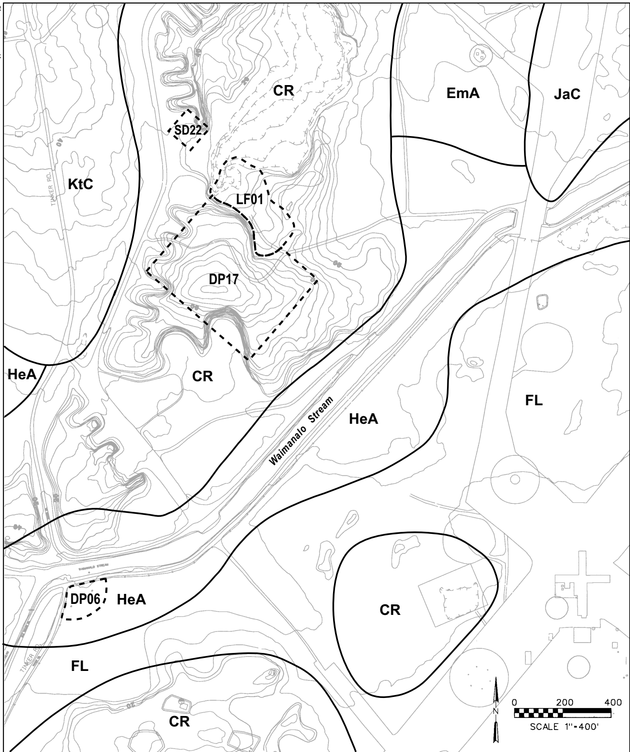
Figure 3-1 Study Area Soil Types and Properties Based on USDA Soil Survey Bellows AFS OU1 EE/CA
