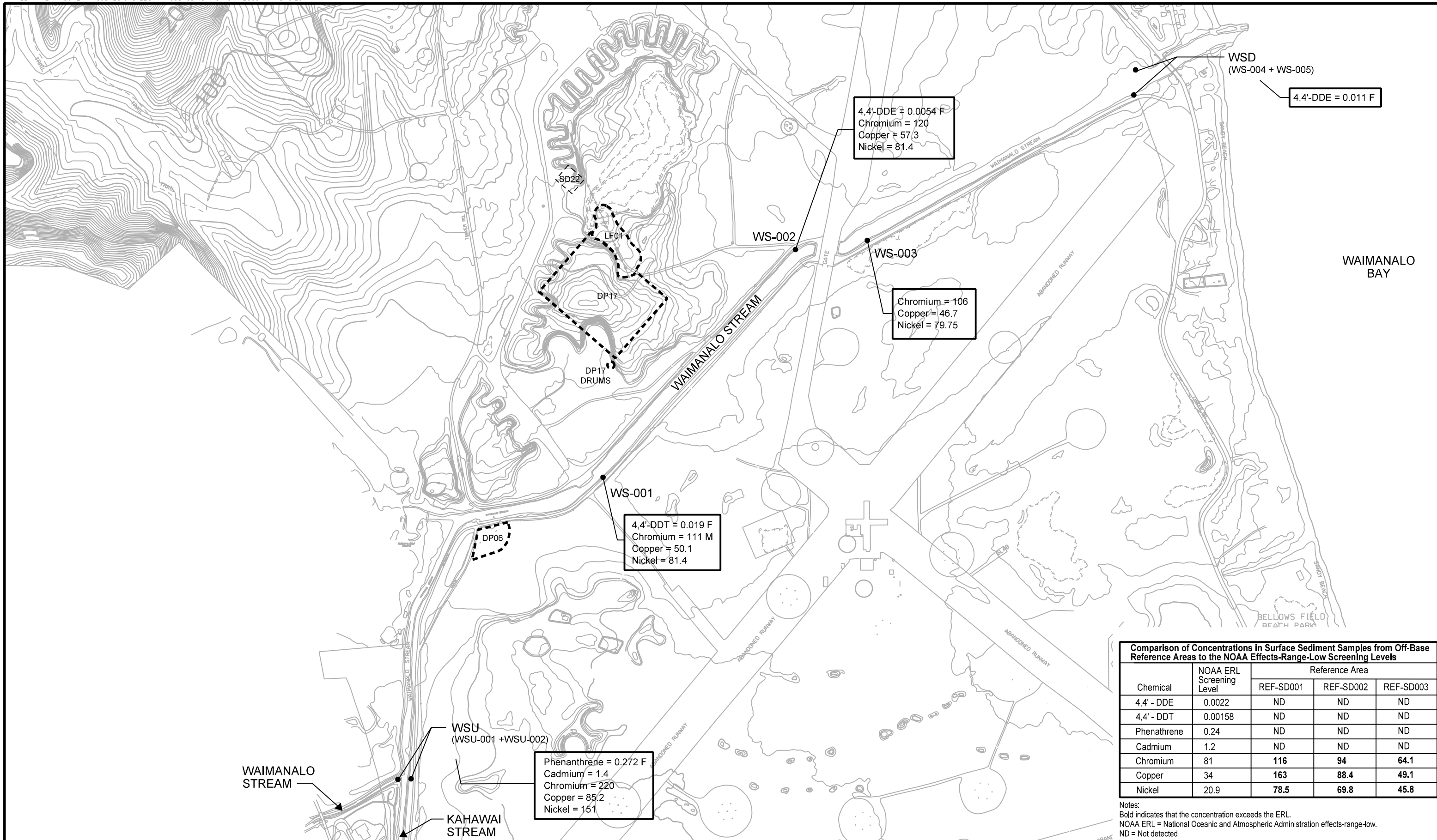
Figure 4-3 Chemicals in Surface Sediments at Concentrations Greater Than NOAA Effects-Range-Low Screening Levels Bellows AFS OU1 EE/CA
