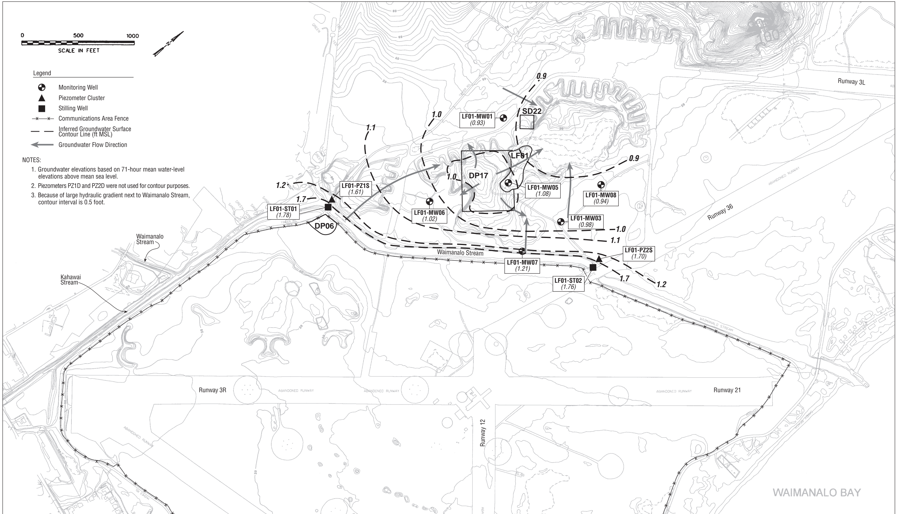
Figure 6 Site LF01: Upper Aquifer Groundwater Contour Map EE/CA FOR SITE LF01, BELLOWS AFS
