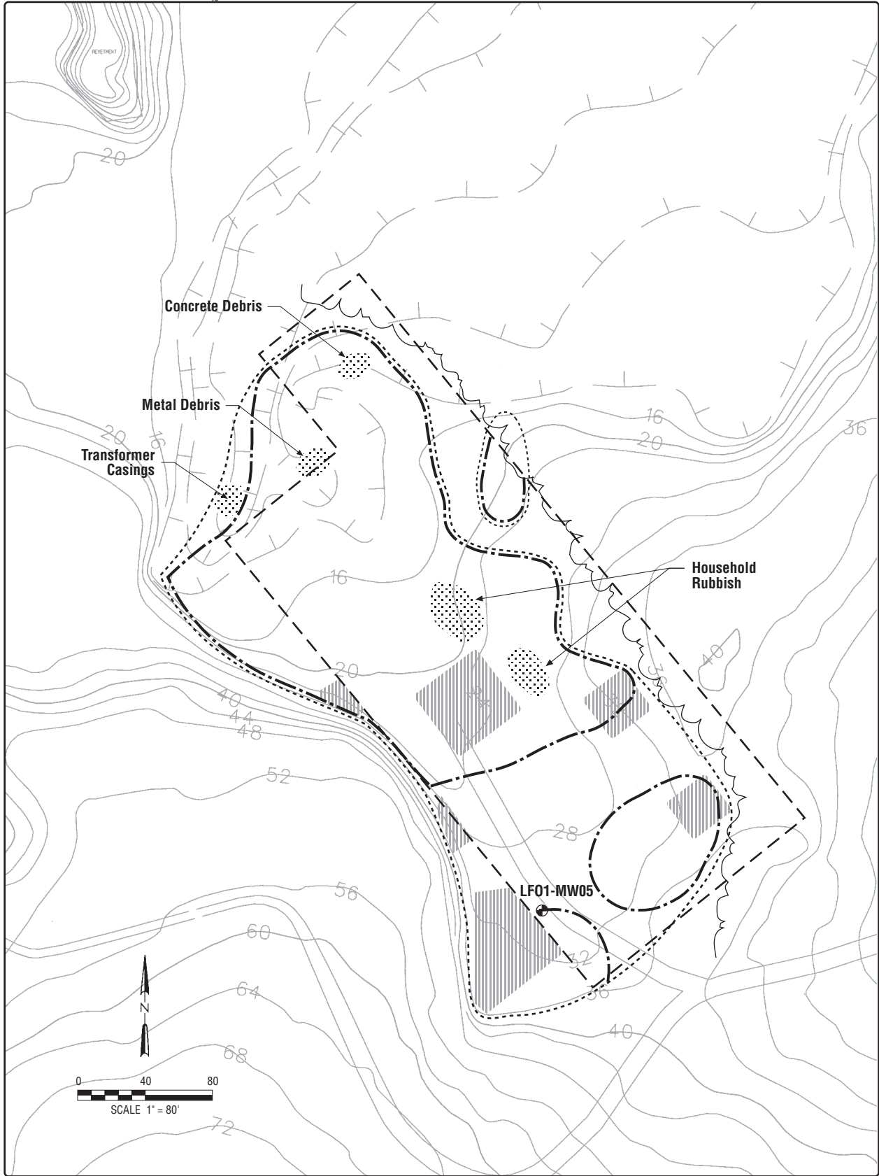
Figure 1-6 Site LF01: Extent and Features Based on EE/CA Pre-Survey Bellows AFS OU1 EE/CA
